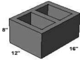
12 x 8 x 16 (305mm x 203mm x 406mm)
