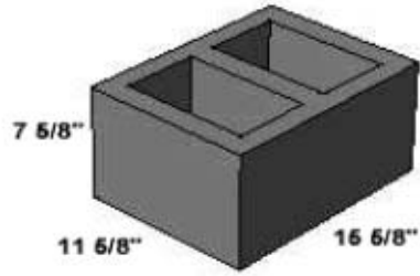
11 5/8 x 7 5/8 x 15 5/8 (295mm x 194mm x 397mm)
