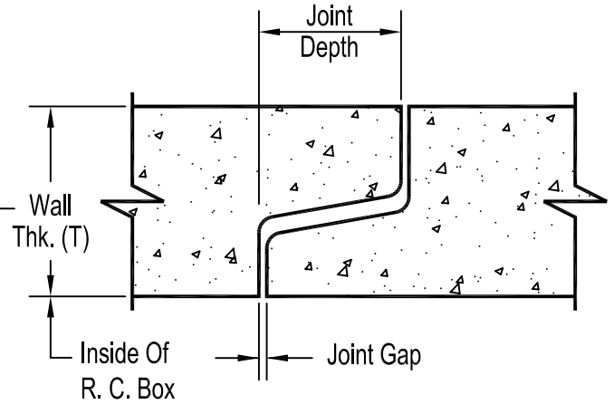
Section thru Box Joint
