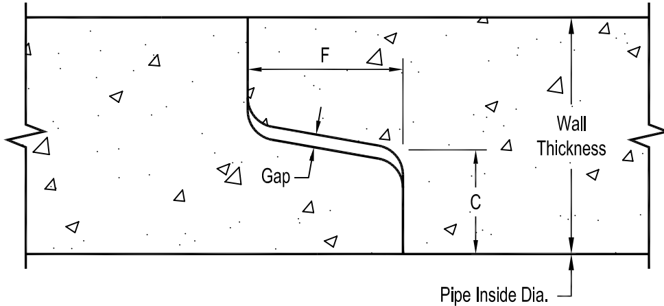
Section Thru Joint
