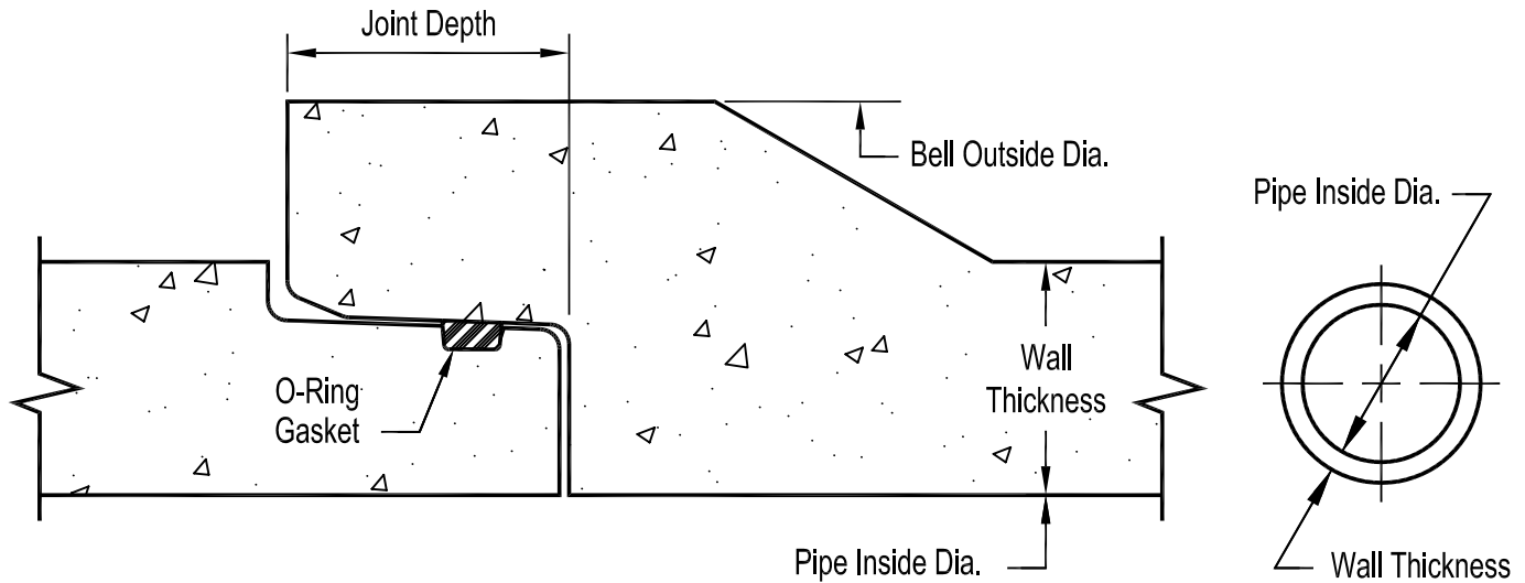
Section Thru Joint
