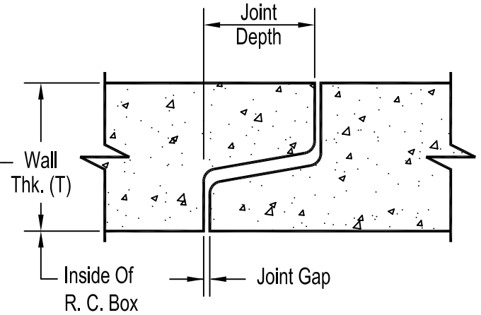
Section thru Box Joint
