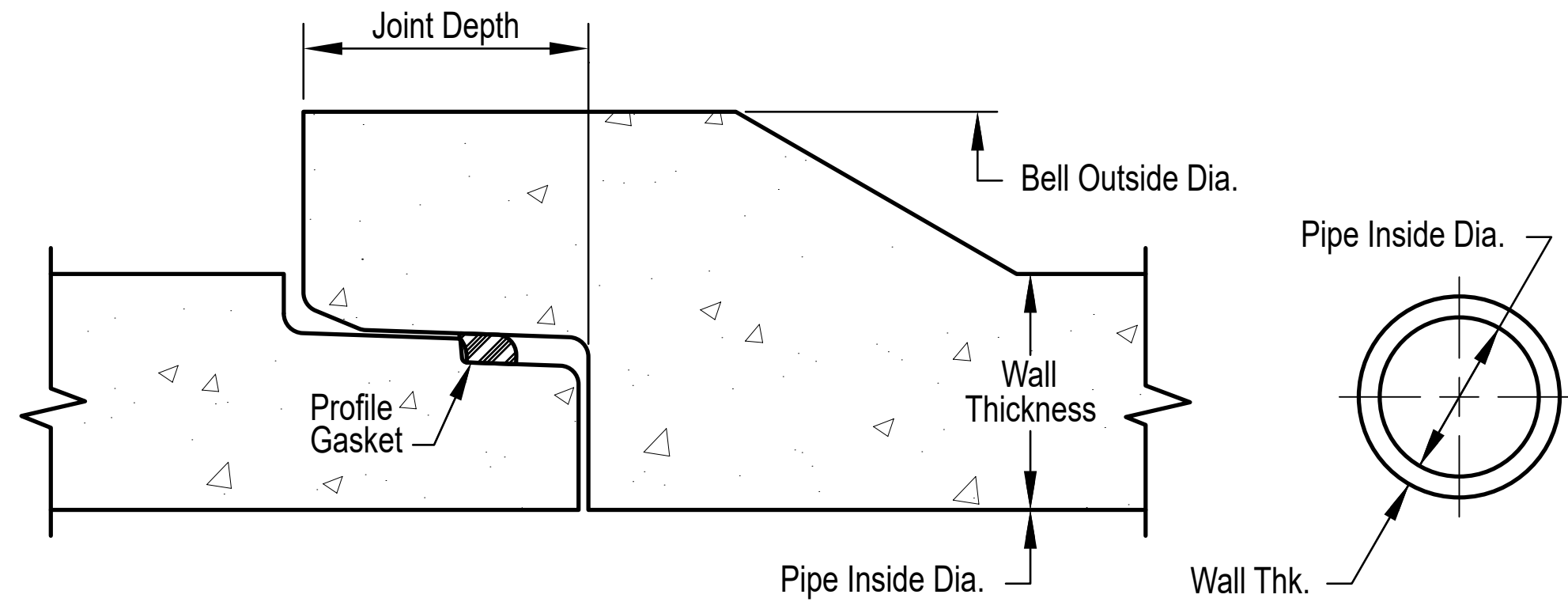
Section Thru Joint
