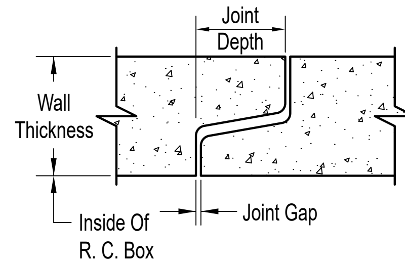
Section thru Box Joint
