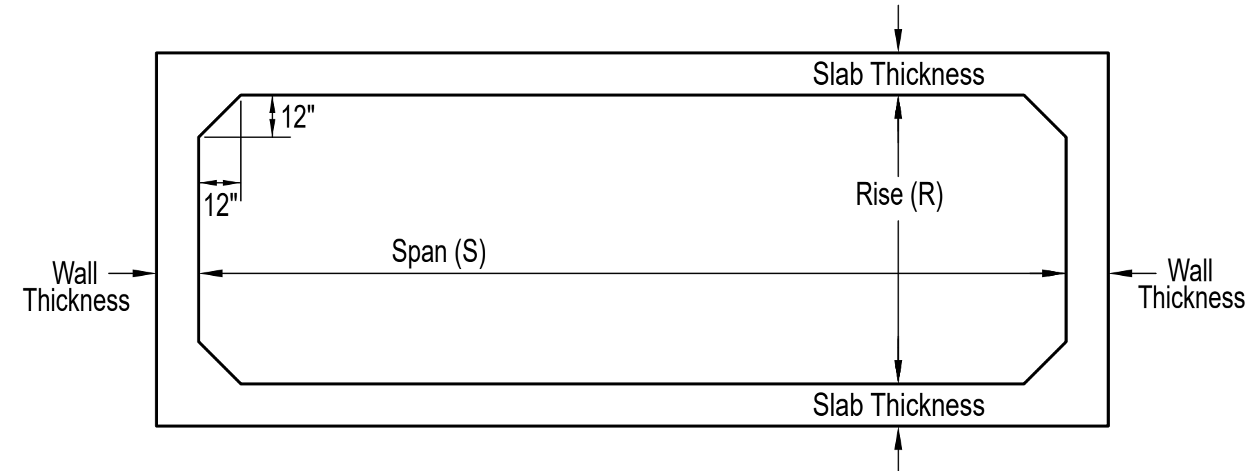
Section thru Box Culvert
