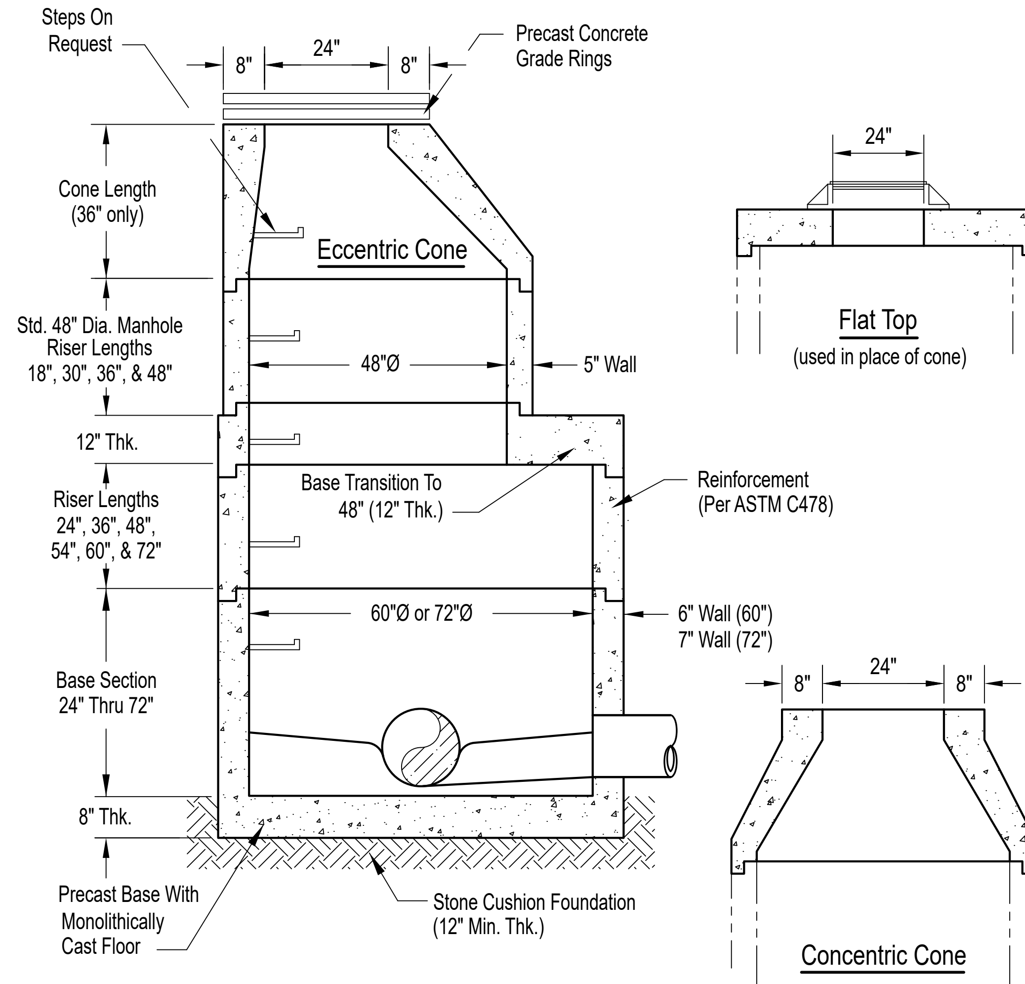
Typical Section Thru Manhole
