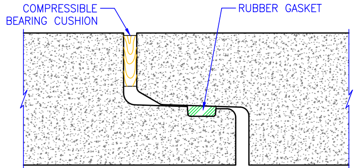
Gasketed Joint
