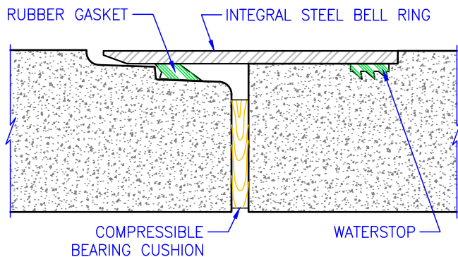
Gasketed Joint with Integral Steel Bell
