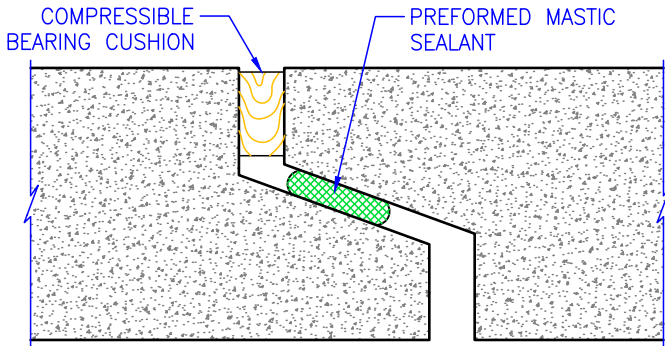
Tongue & Groove Joint
