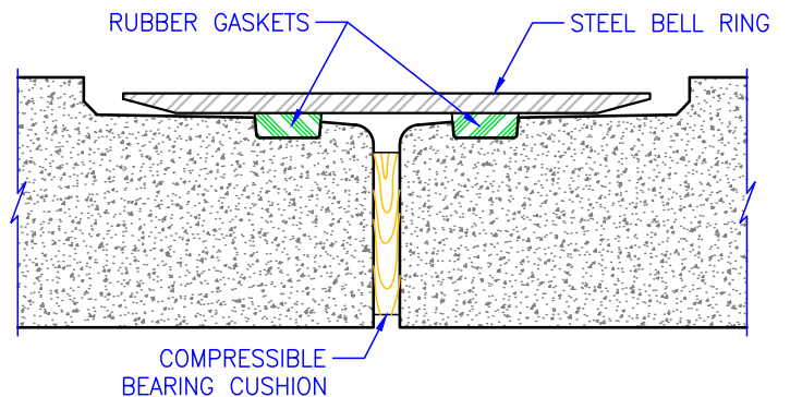
Gasketed Joint with Steel Bell
