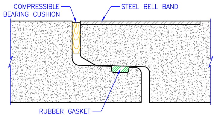
Gasketed Joint with Steel Bell Band
