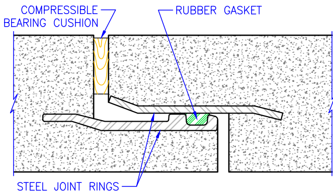
Gasketed Steel Ring Joint
