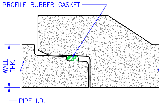
Section Thru Joint
