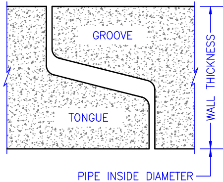
Section Thru Joint
