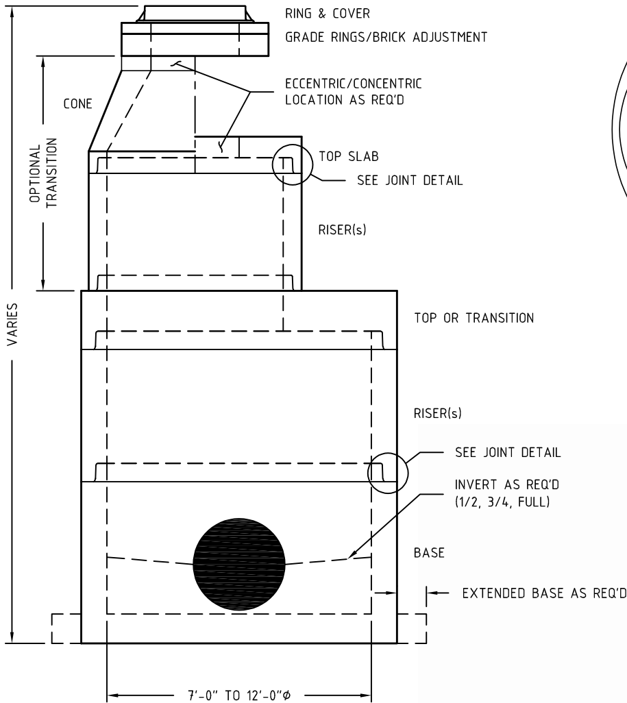
Elevation View
